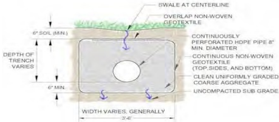
Figure B-4: Typical Infiltration Trench
