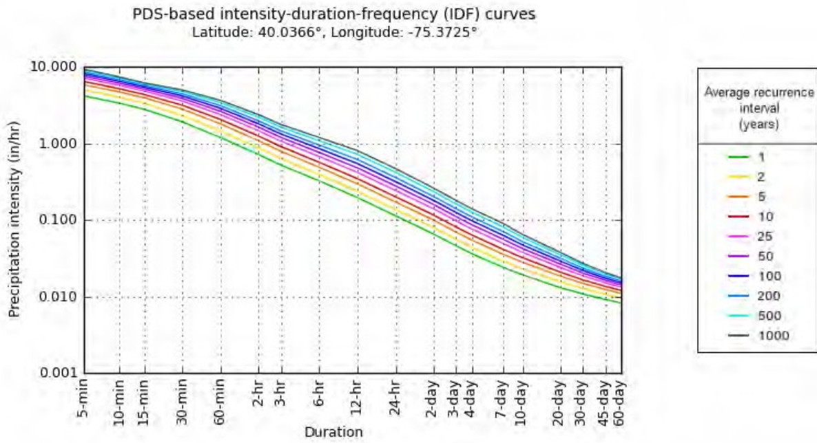
FIGURE F-1 INTENSITY-DURATION-FREQUENCY (DDF) CURVES
